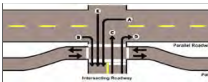
FIGURE 7-3 INTERSECTION DESIGN METHODS TO REDUCE SIDEPath CONFLICTS
