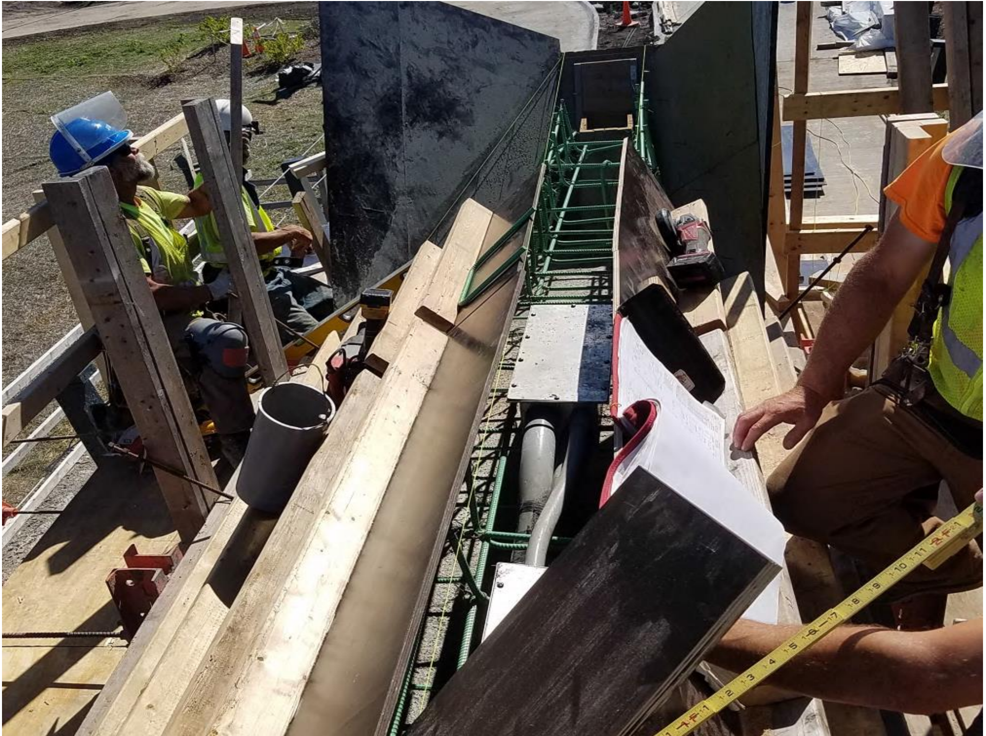
July 23, 2020- Contractor forming cornice and installing reinforcements
