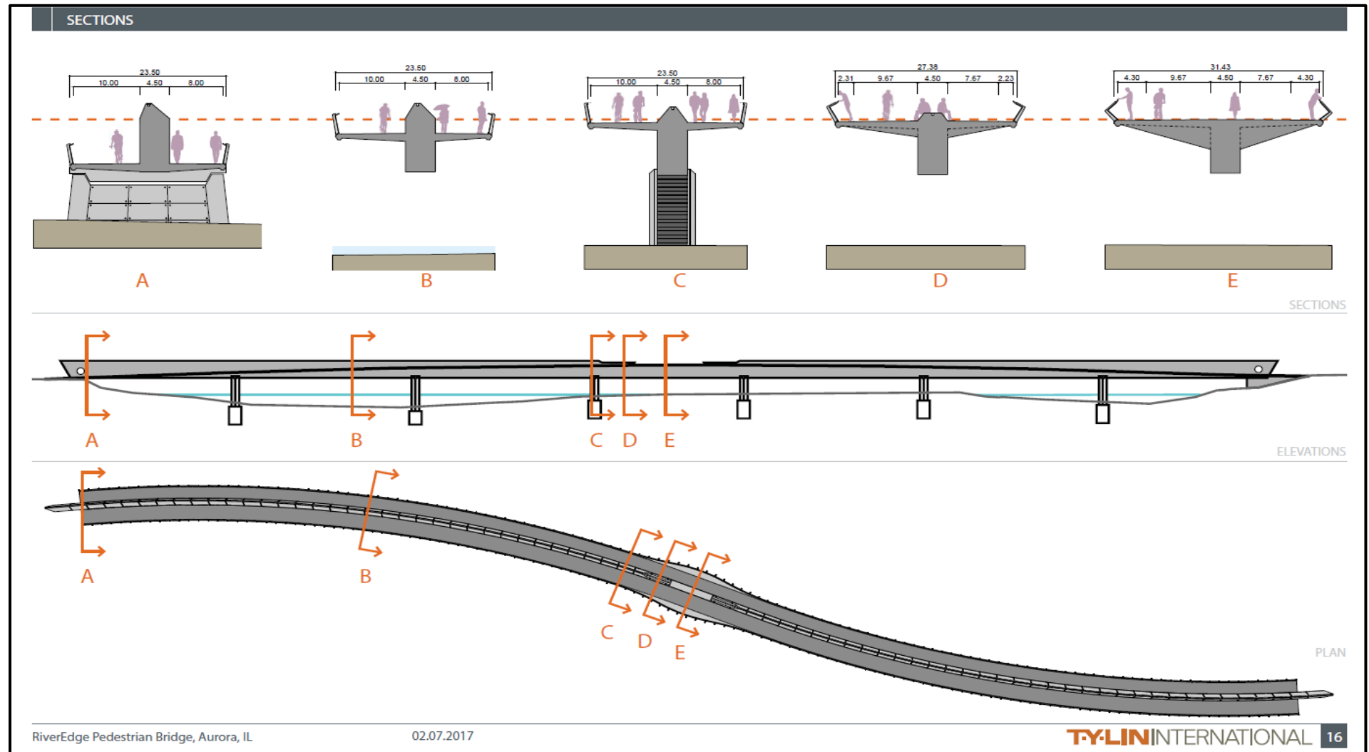
Cross-sections of bridge.
