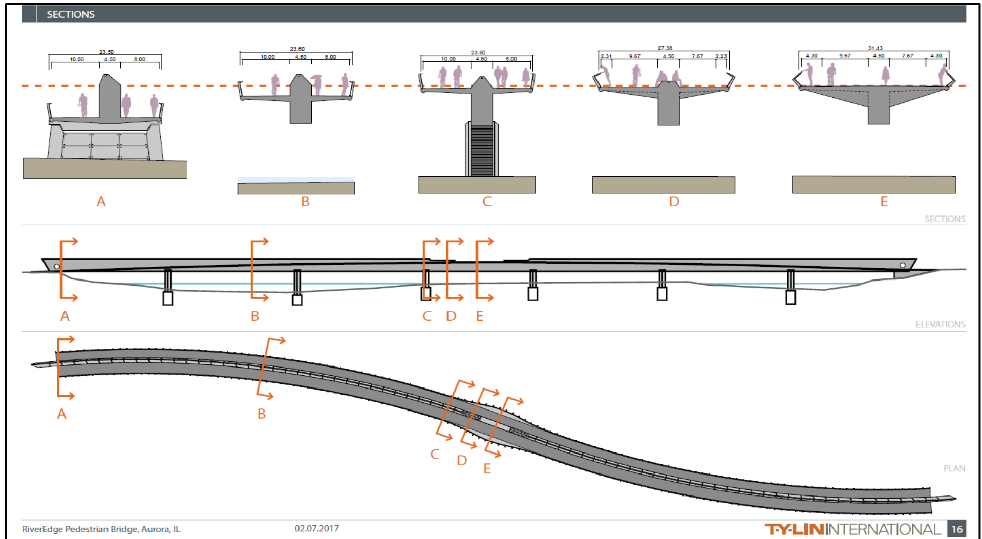
Cross-sections of bridge.
