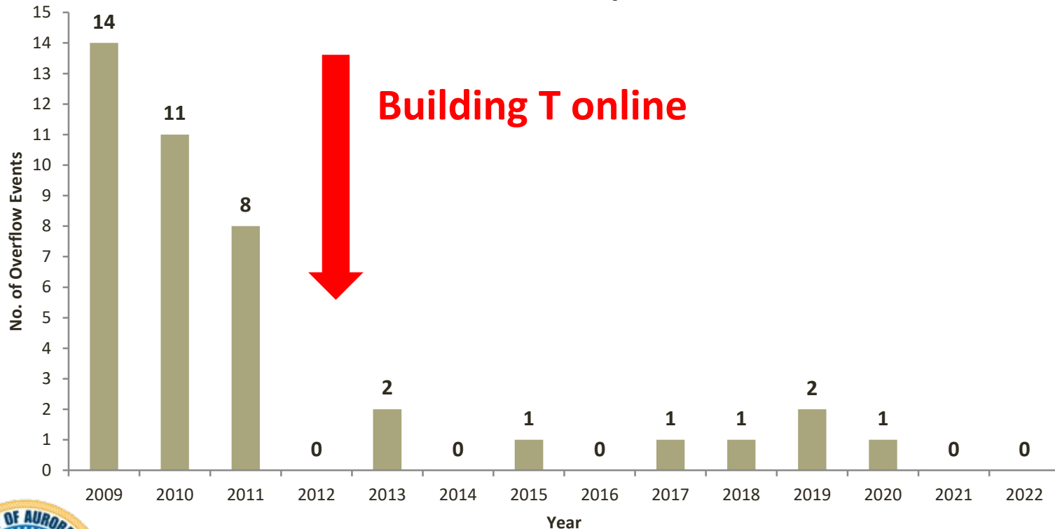
Annual Overflow Events per Year: 2009-2022
